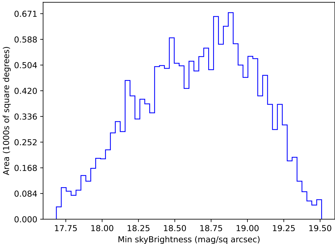
weather_cloudso35v3.4_10yrs WFD r band: Min skyBrightness
