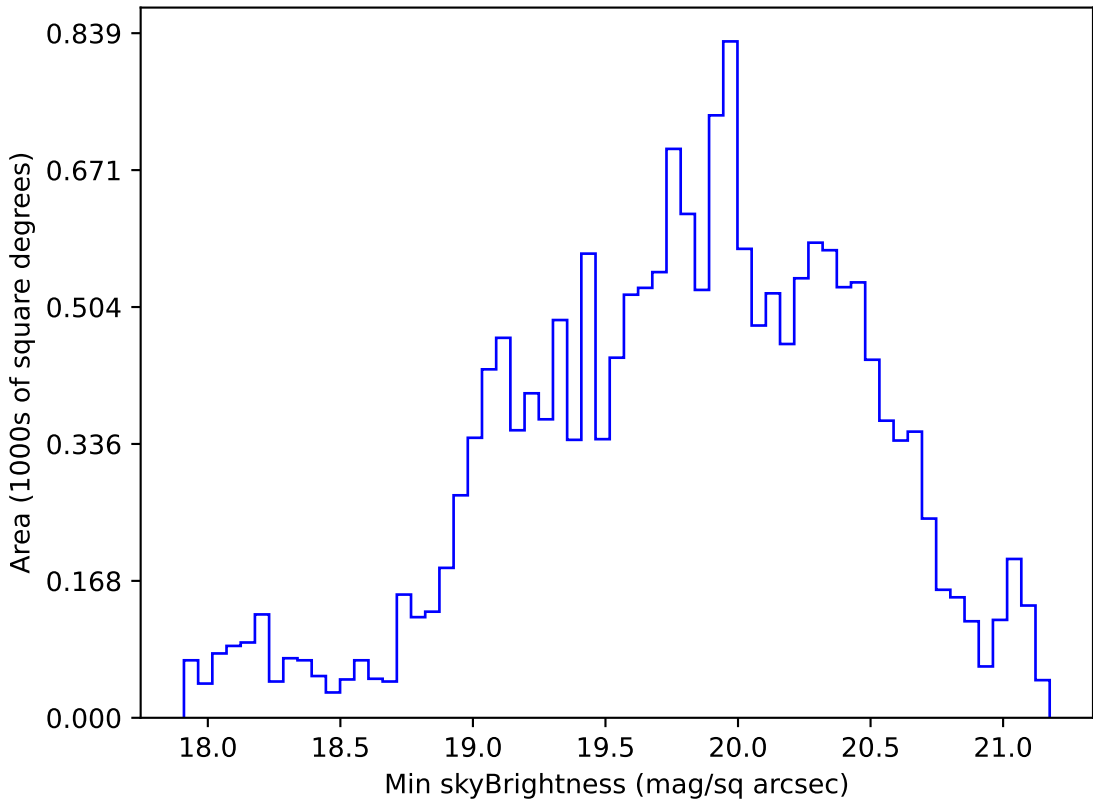
weather_cloudso35v3.4_10yrs WFD g band: Min skyBrightness
