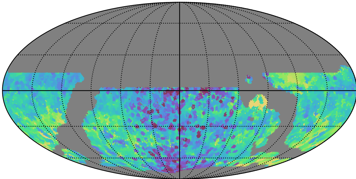
weather_cloudso35v3.4_10yrs WFD all bands: Min skyBrightness
