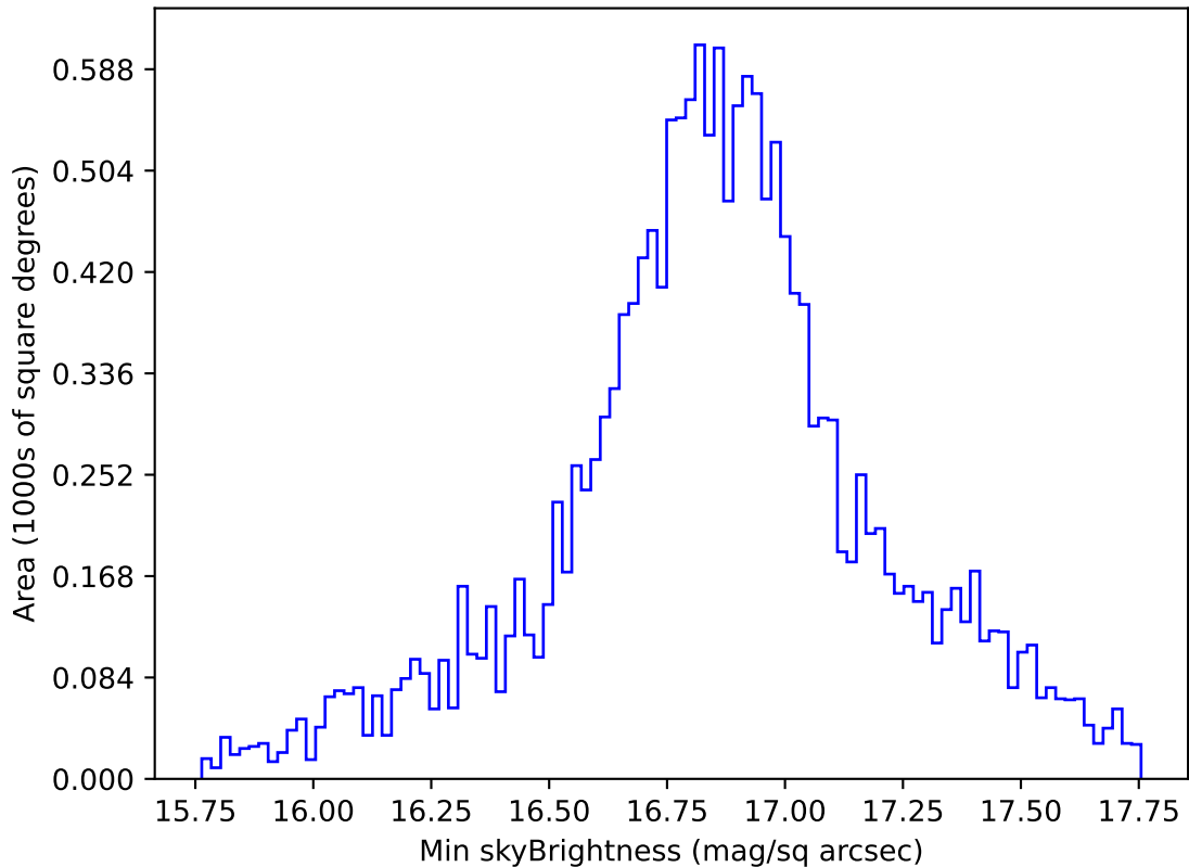
weather_cloudso35v3.4_10yrs WFD all bands: Min skyBrightness
