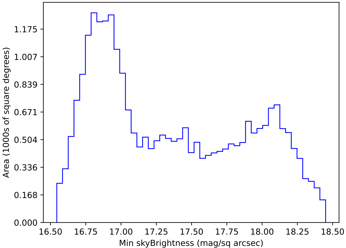
weather_cloudso35v3.4_10yrs All sky z band: Min skyBrightness
