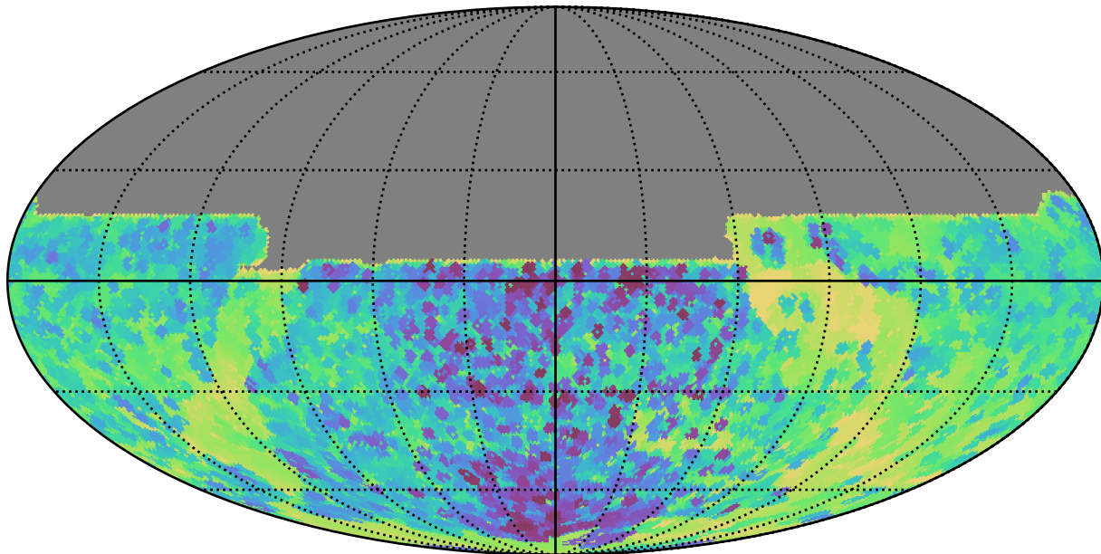
weather_cloudso35v3.4_10yrs All sky y band: Min skyBrightness
