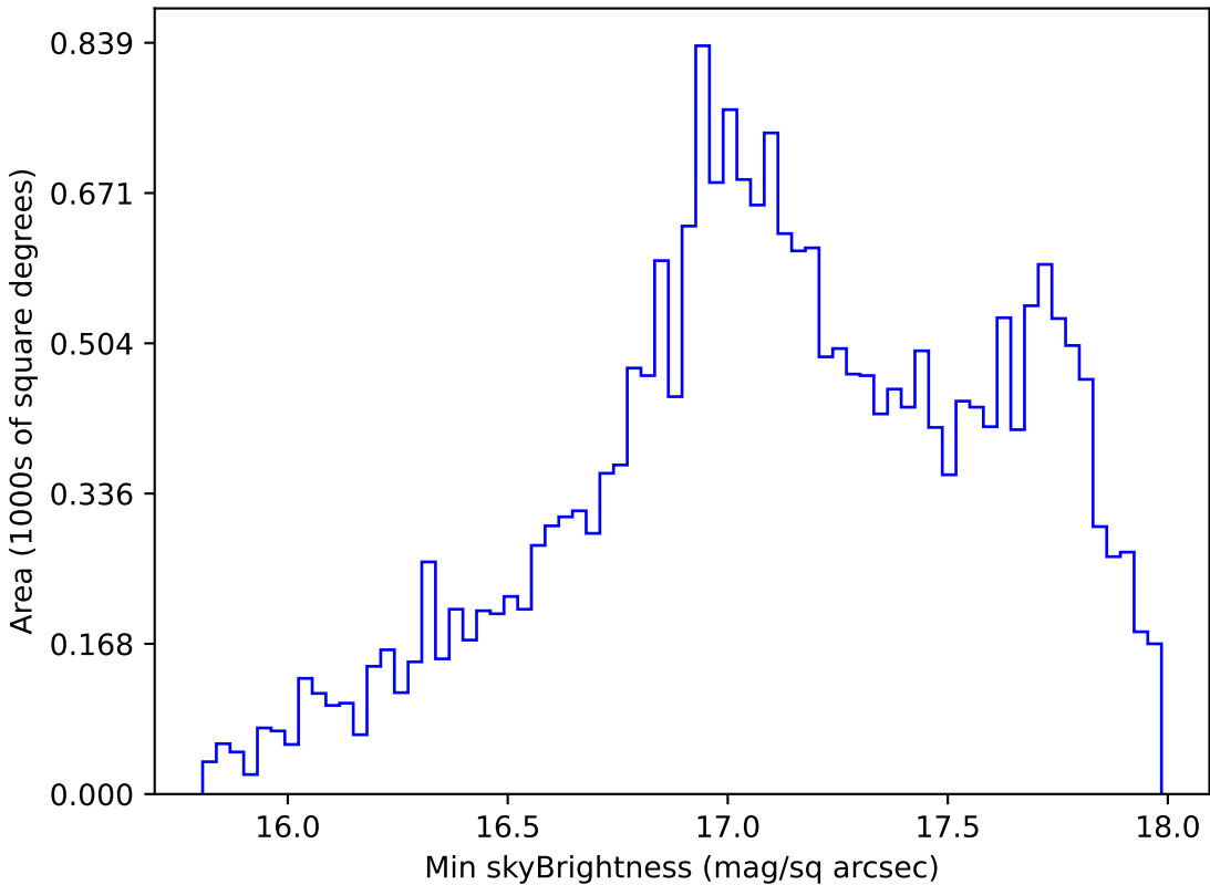
weather_cloudso35v3.4_10yrs All sky y band: Min skyBrightness
