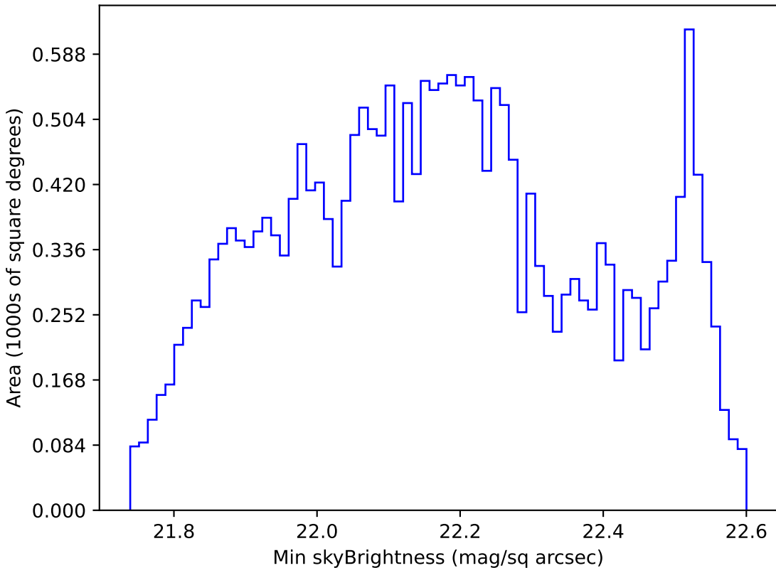
weather_cloudso35v3.4_10yrs All sky u band: Min skyBrightness
