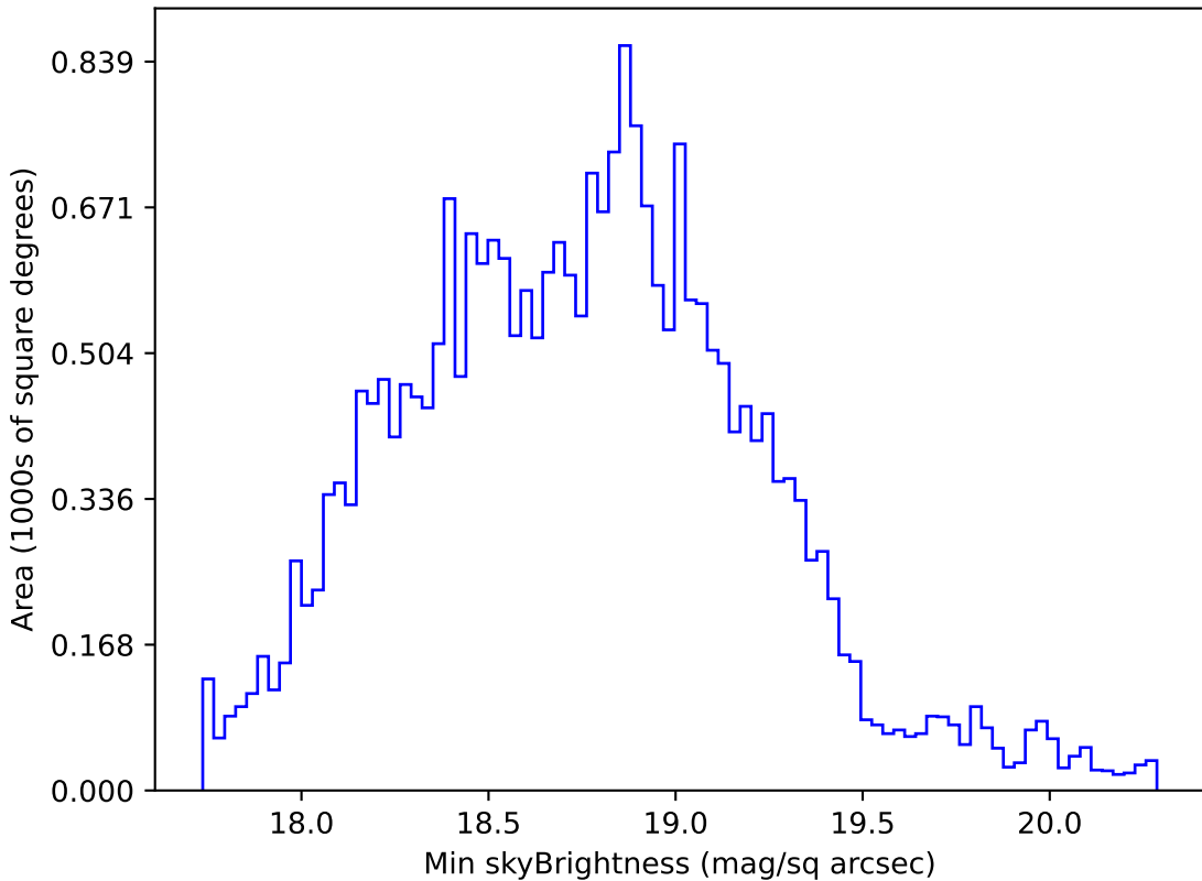
weather_cloudso35v3.4_10yrs All sky r band: Min skyBrightness
