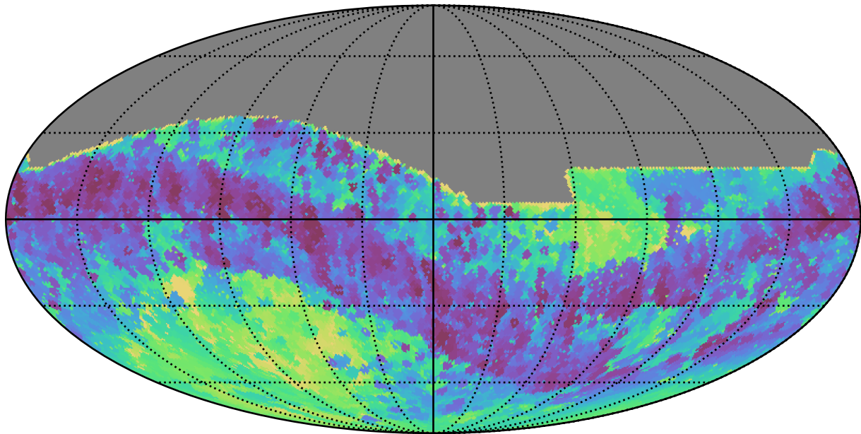
weather_cloudso35v3.4_10yrs All sky i band: Min skyBrightness
