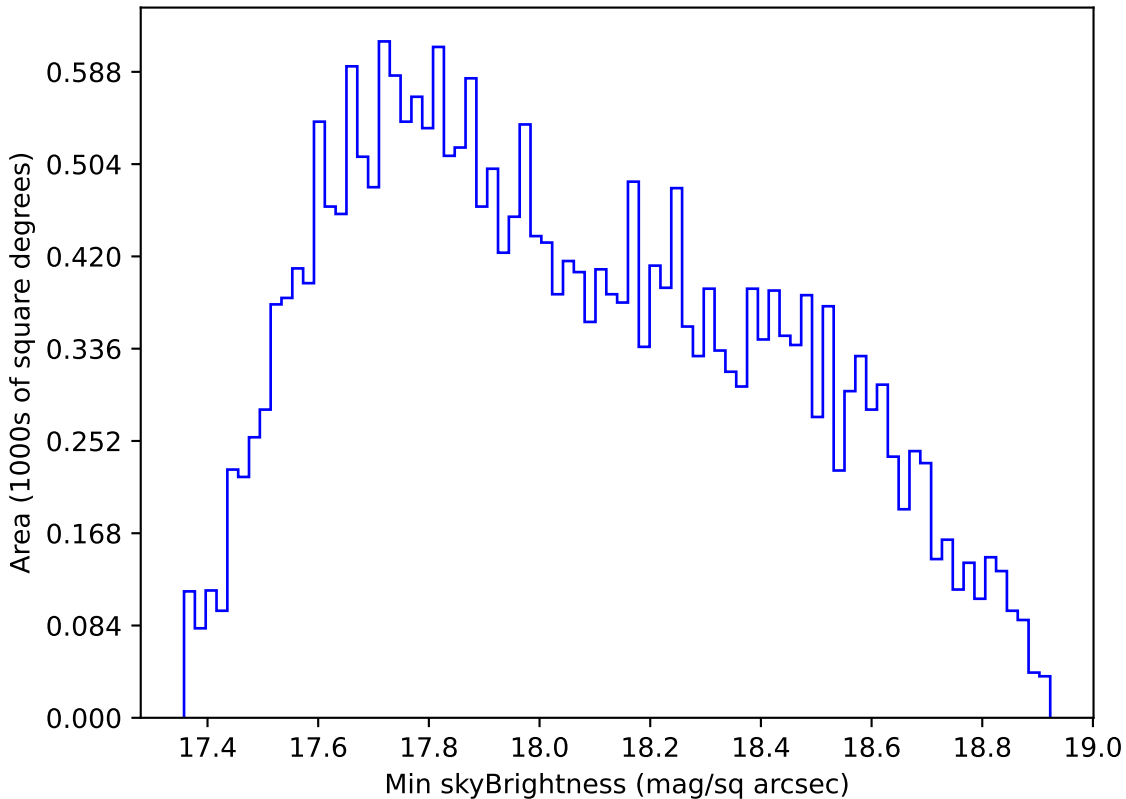
weather_cloudso35v3.4_10yrs All sky i band: Min skyBrightness
