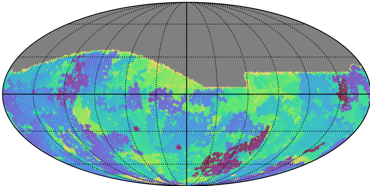
weather_cloudso35v3.4_10yrs All sky g band: Min skyBrightness
