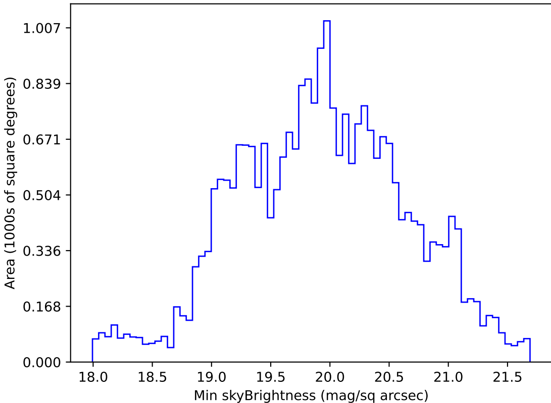
weather_cloudso35v3.4_10yrs All sky g band: Min skyBrightness
