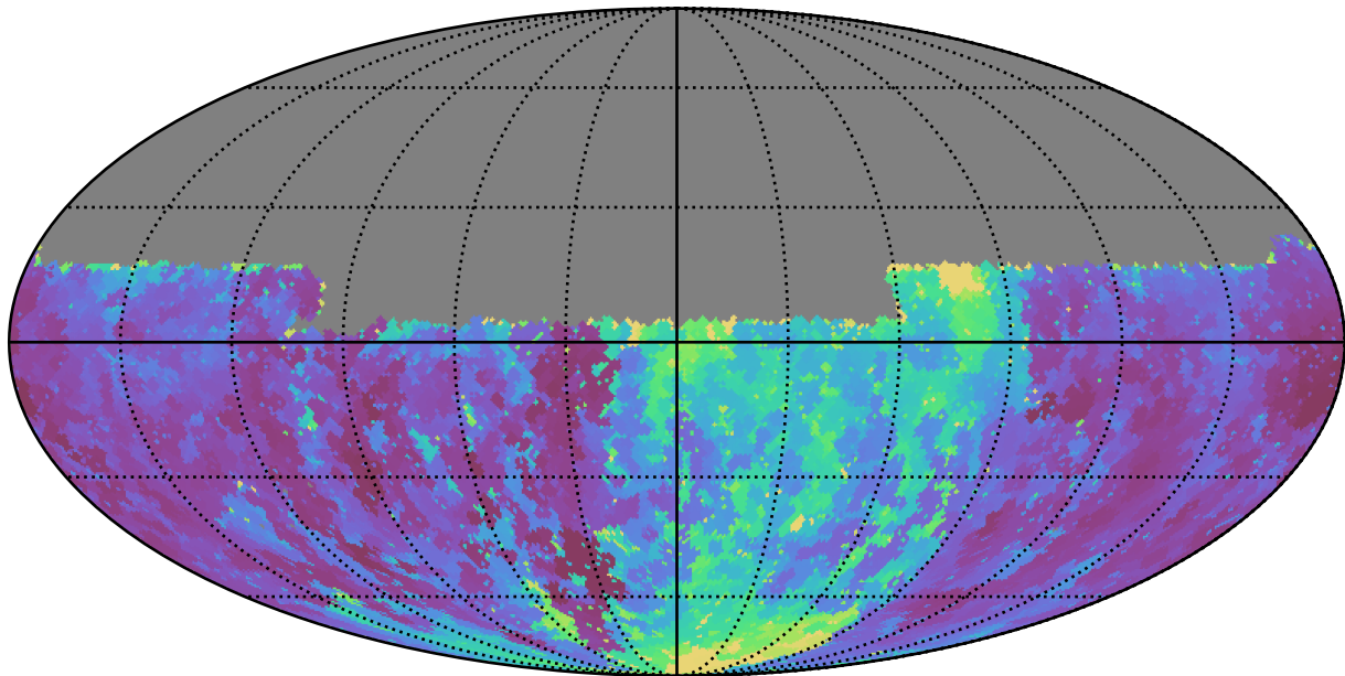
weather_cloudso35v3.4_10yrs Yr 1 u band: Min seeingGeom
