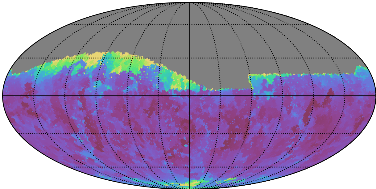
weather_cloudso35v3.4_10yrs Yr 1 r band: Min seeingGeom
