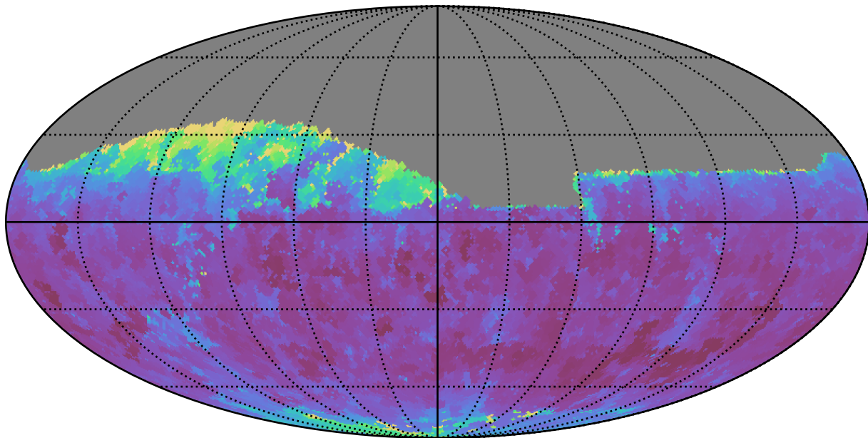
weather_cloudso35v3.4_10yrs Yr 1 i band: Min seeingEff
