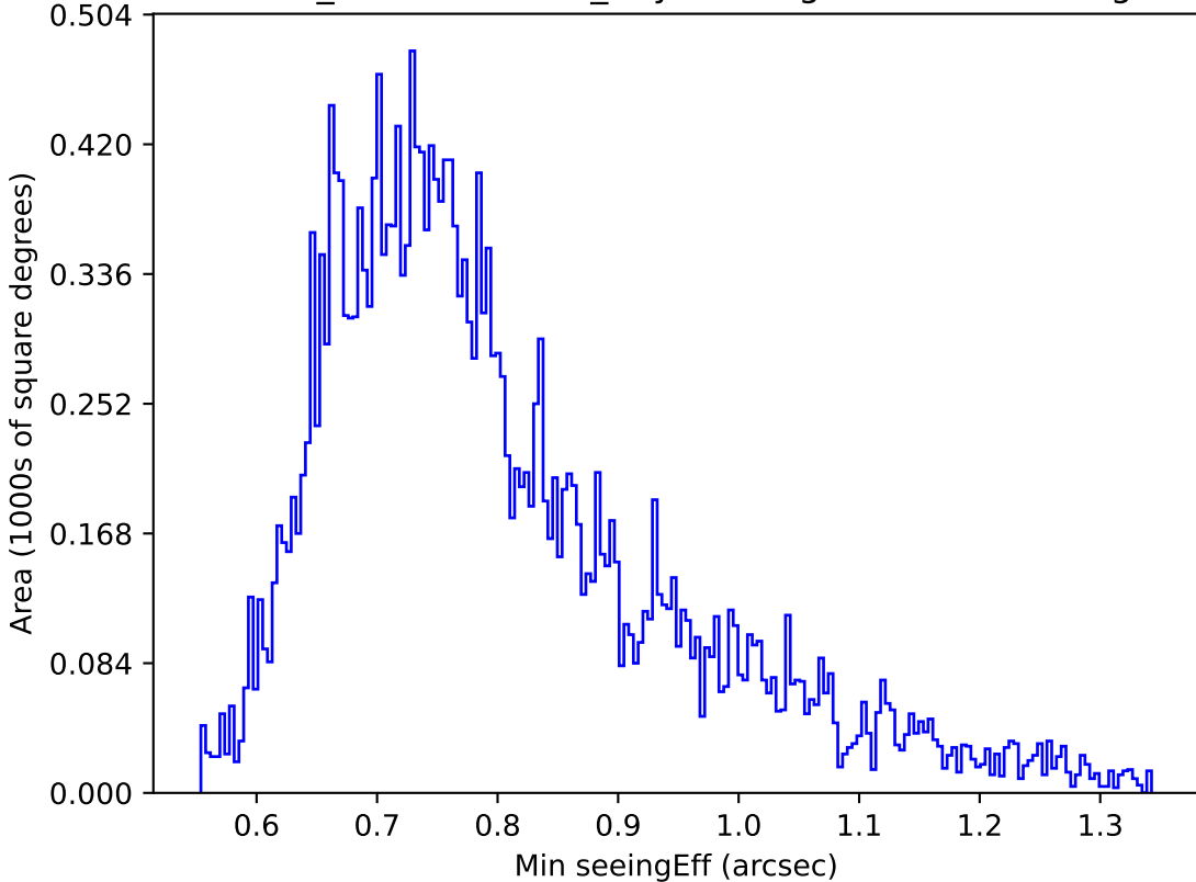
weather_cloudso35v3.4_10yrs Yr 1 g band: Min seeingEff
