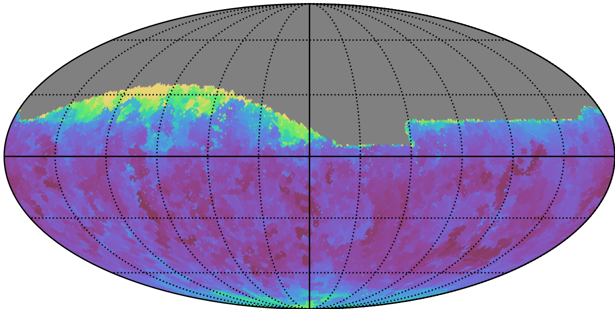
weather_cloudso35v3.4_10yrs Yr 1 all bands: Min seeingEff
