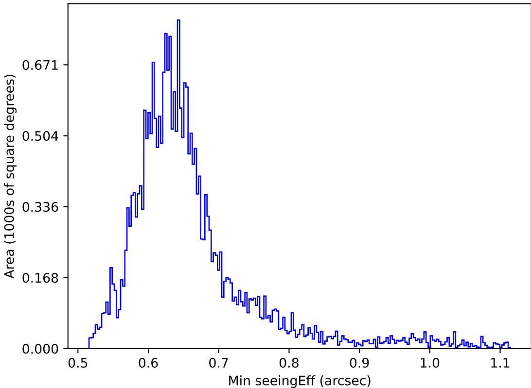
weather_cloudso35v3.4_10yrs Yr 1 all bands: Min seeingEff
