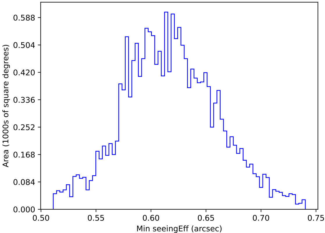
weather_cloudso35v3.4_10yrs WFD z band: Min seeingEff
