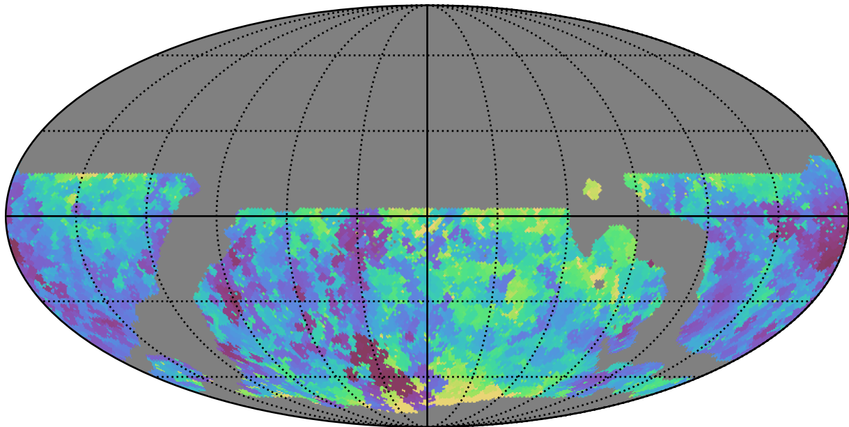
weather_cloudso35v3.4_10yrs WFD u band: Min seeingEff
