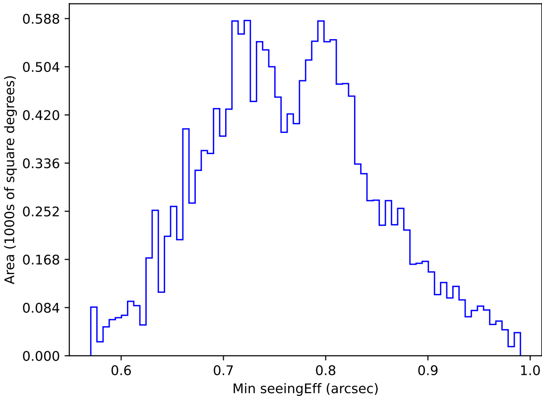
weather_cloudso35v3.4_10yrs WFD u band: Min seeingEff
