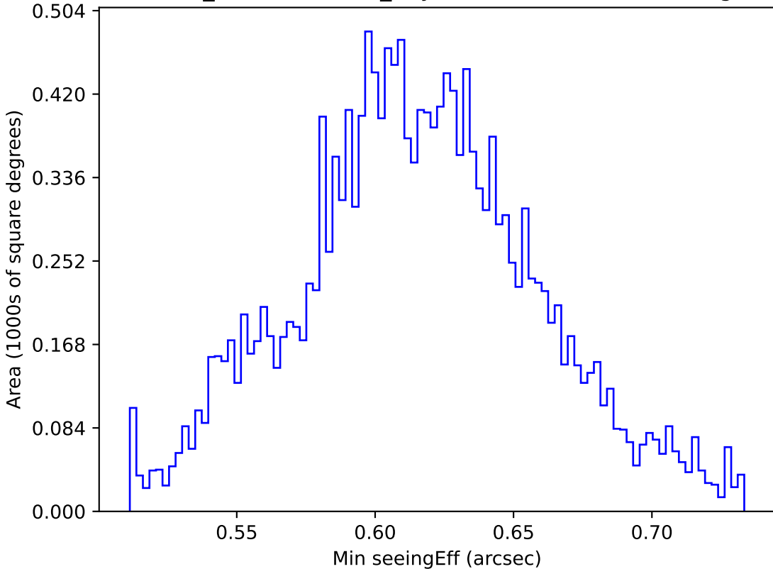
weather_cloudso35v3.4_10yrs WFD r band: Min seeingEff
