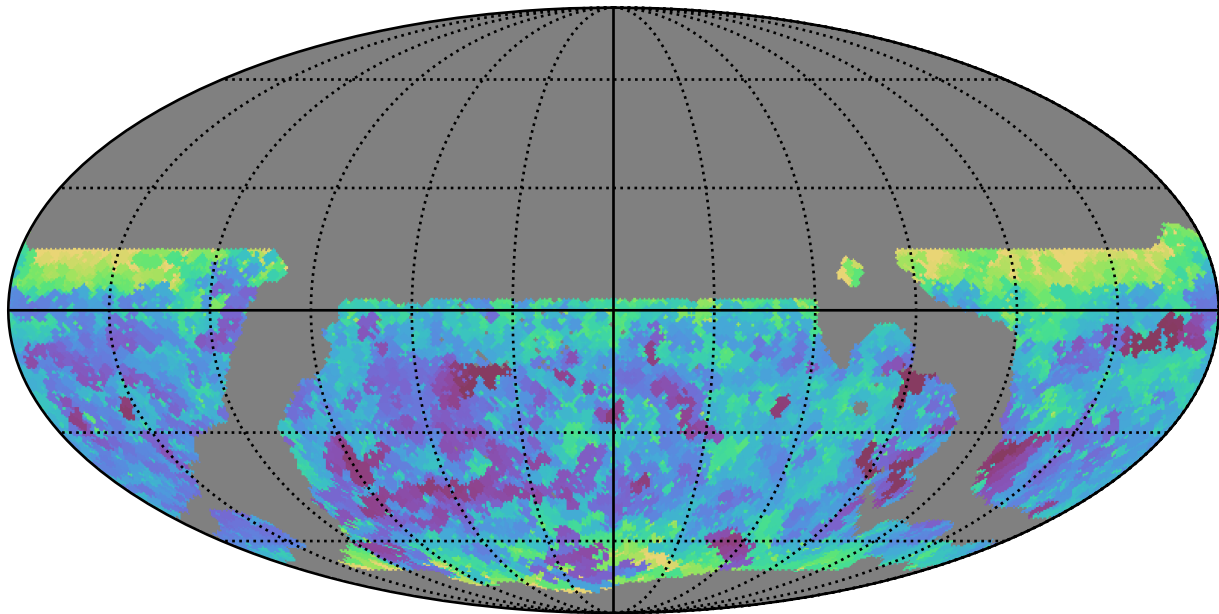
weather_cloudso35v3.4_10yrs WFD i band: Min seeingEff
