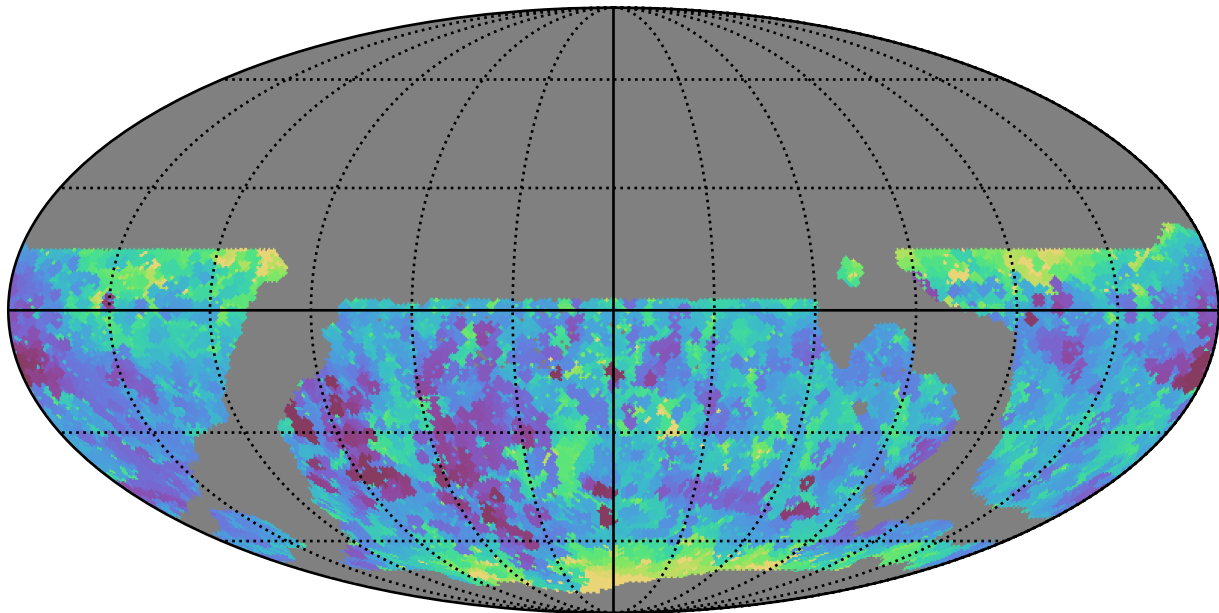
weather_cloudso35v3.4_10yrs WFD g band: Min seeingEff
