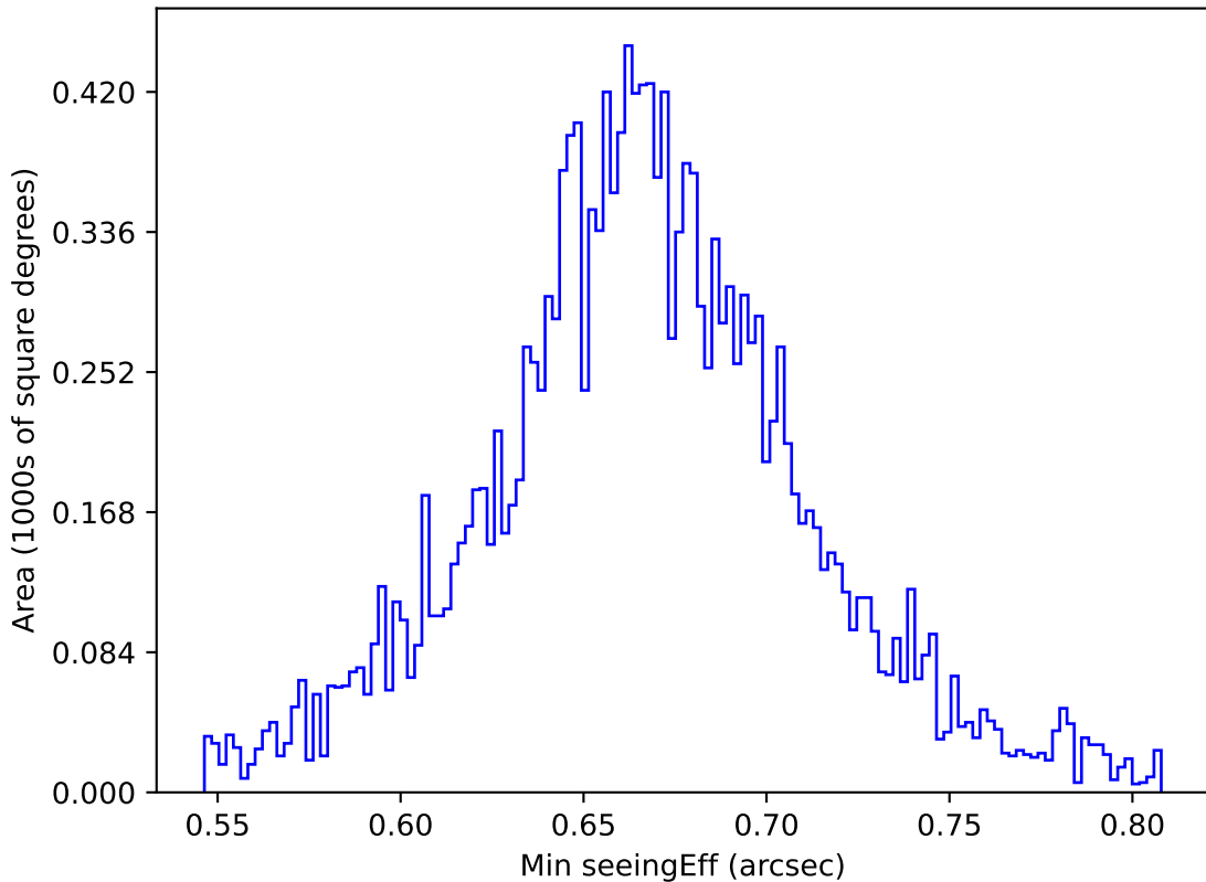
weather_cloudso35v3.4_10yrs WFD g band: Min seeingEff
