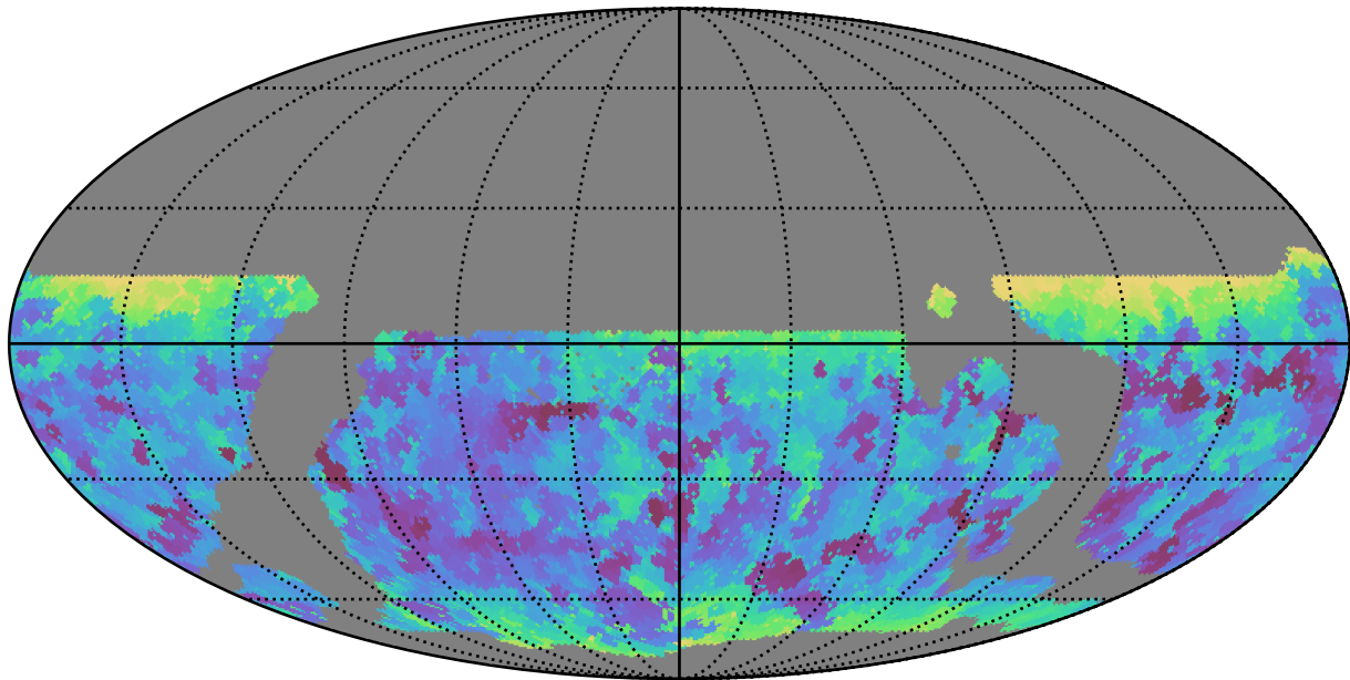
weather_cloudso35v3.4_10yrs WFD all bands: Min seeingEff
