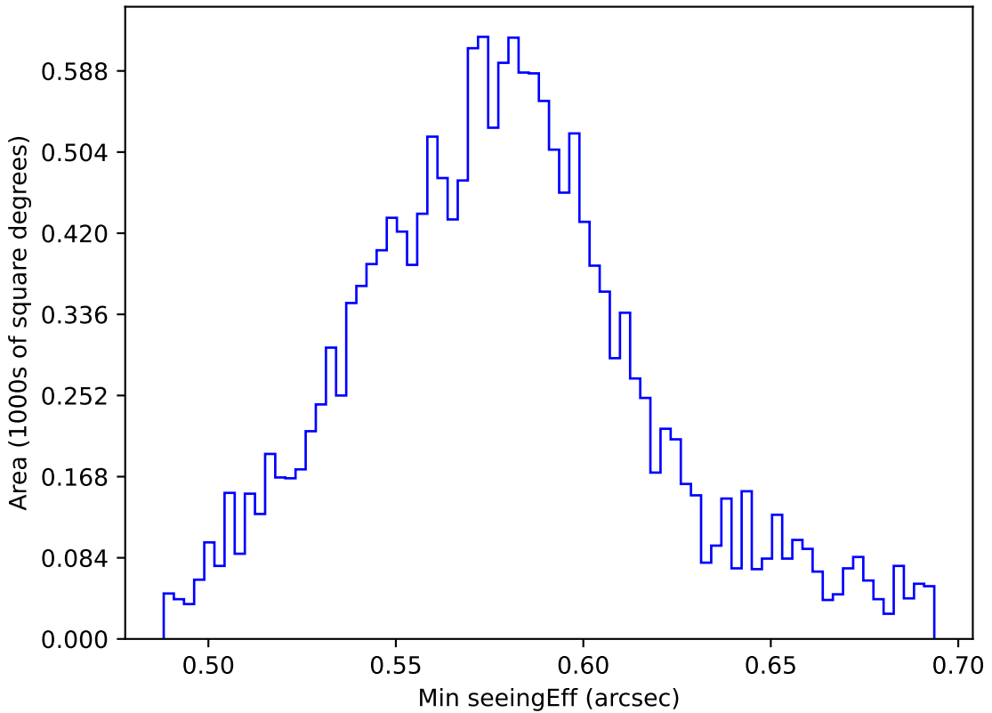
weather_cloudso35v3.4_10yrs WFD all bands: Min seeingEff
