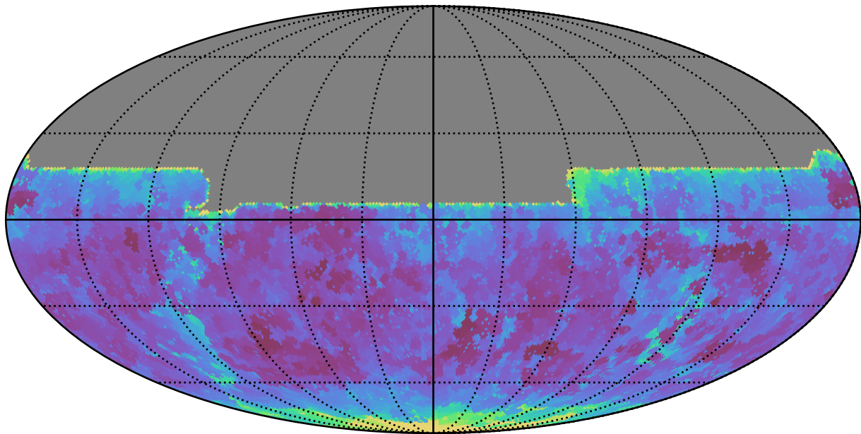
weather_cloudso35v3.4_10yrs All sky y band: Min seeingEff
