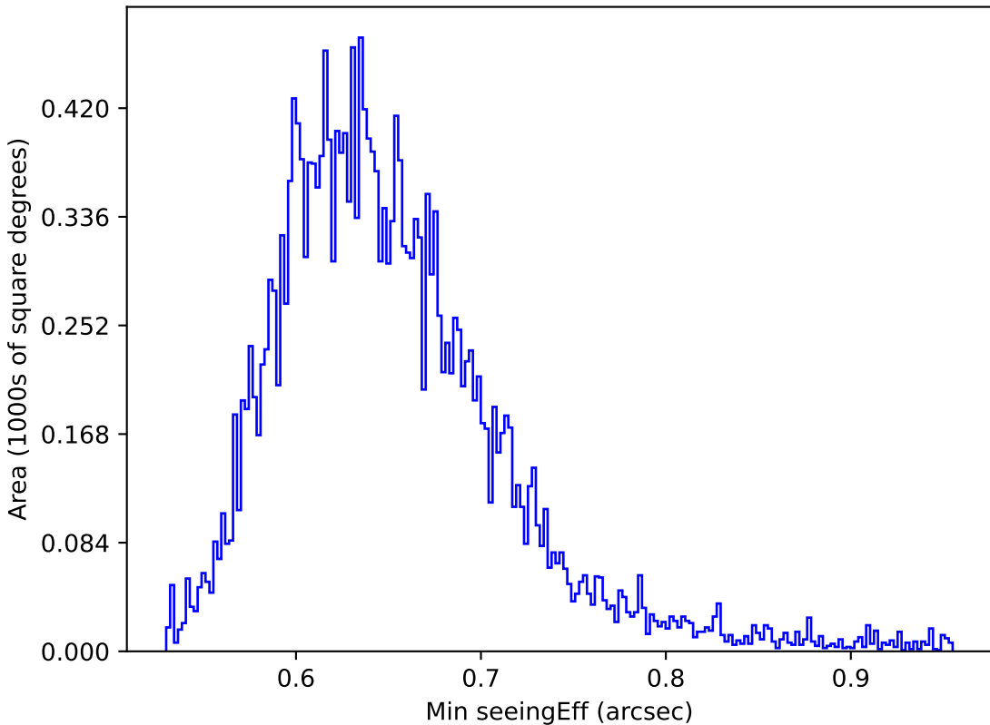
weather_cloudso35v3.4_10yrs All sky y band: Min seeingEff
