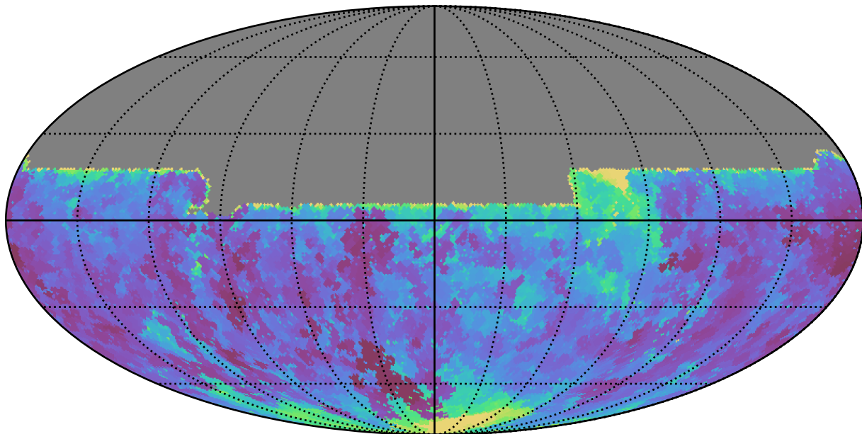
weather_cloudso35v3.4_10yrs All sky u band: Min seeingEff
