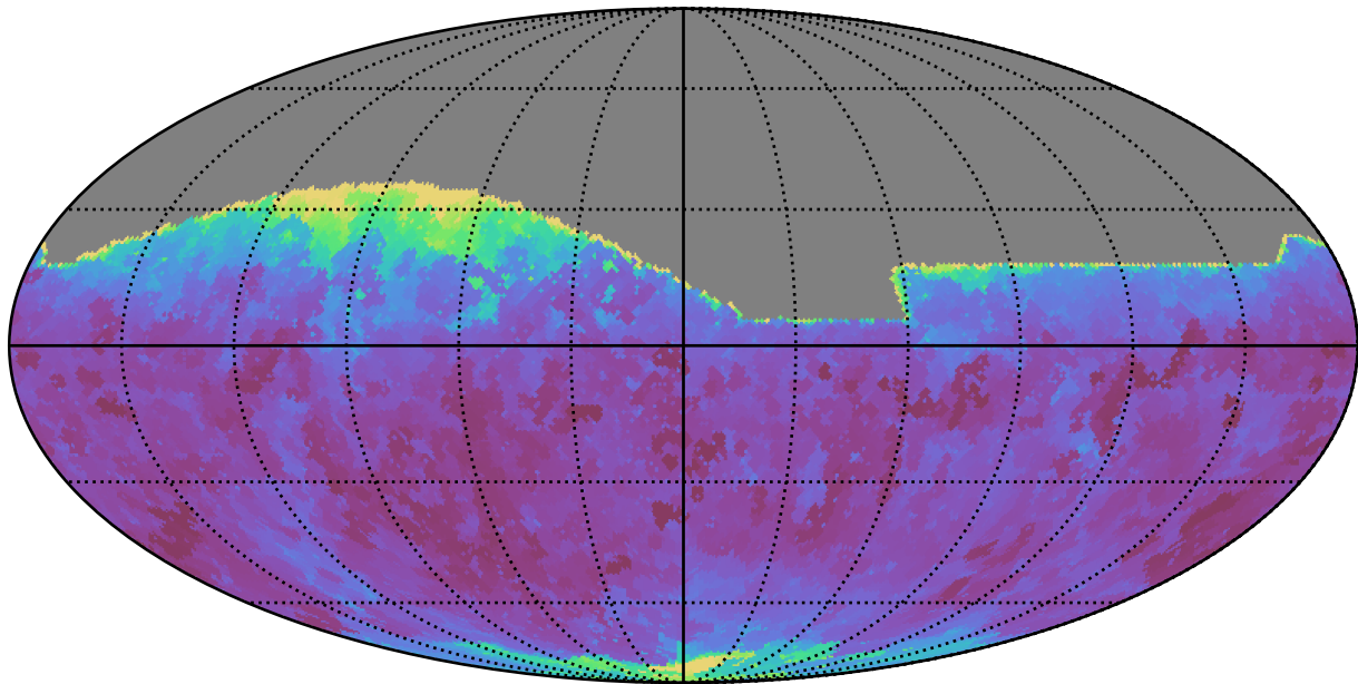
weather_cloudso35v3.4_10yrs All sky r band: Min seeingEff
