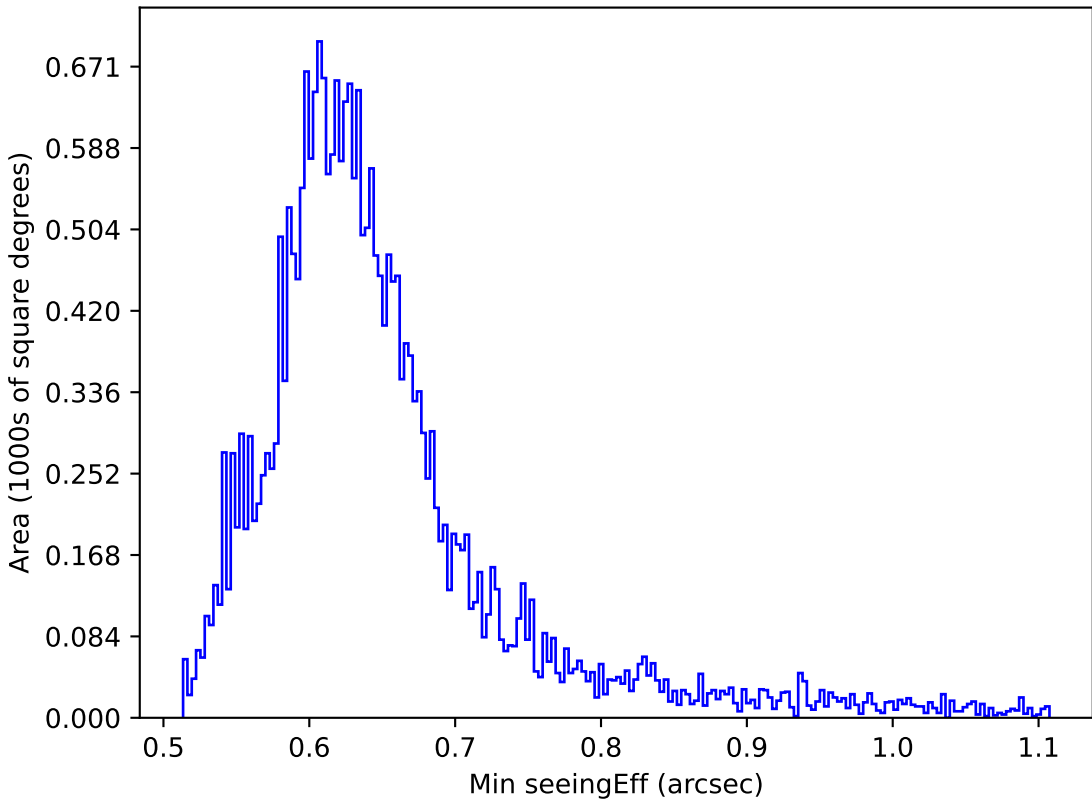
weather_cloudso35v3.4_10yrs All sky r band: Min seeingEff
