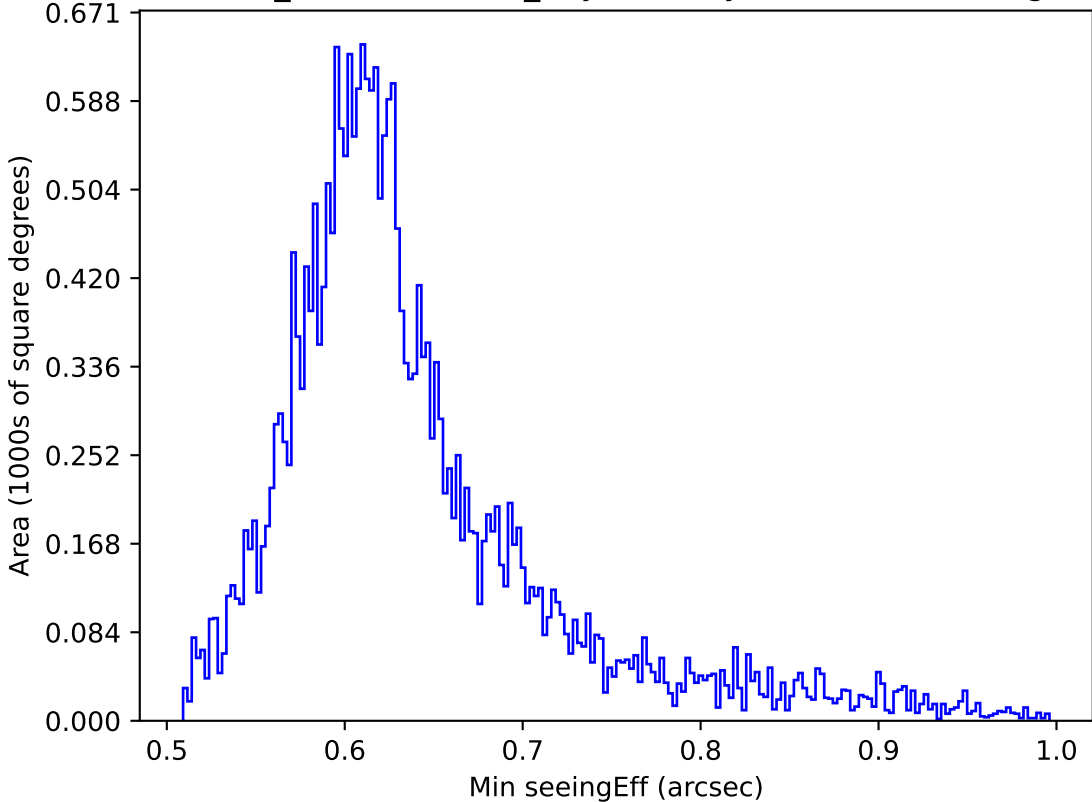
weather_cloudso35v3.4_10yrs All sky i band: Min seeingEff
