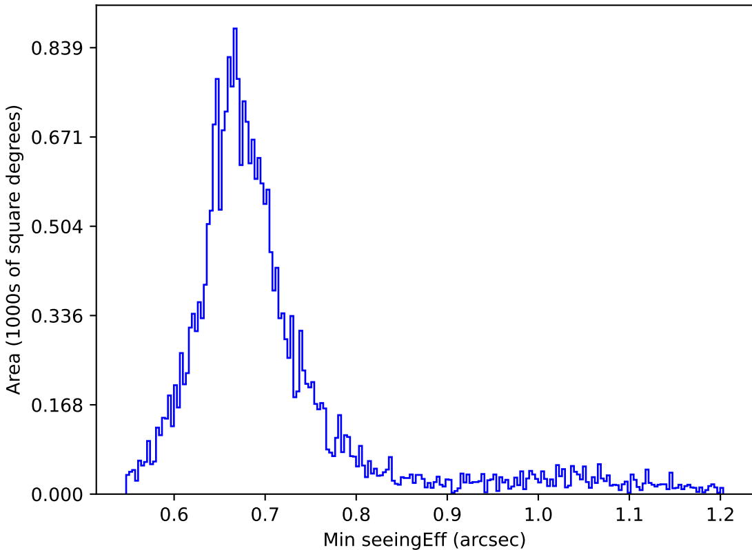
weather_cloudso35v3.4_10yrs All sky g band: Min seeingEff
