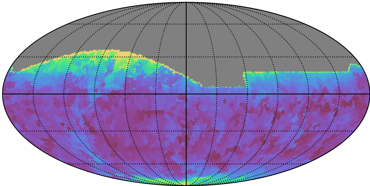
weather_cloudso35v3.4_10yrs All sky all bands: Min seeingEff
