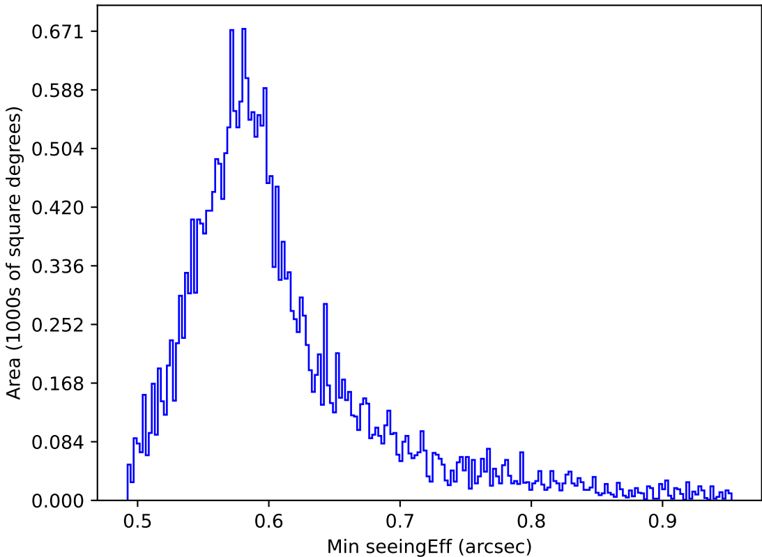
weather_cloudso35v3.4_10yrs All sky all bands: Min seeingEff
