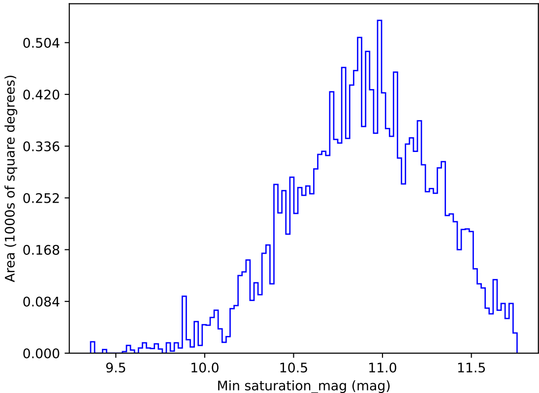
weather_cloudso35v3.4_10yrs WFD all bands: Min saturation_mag
