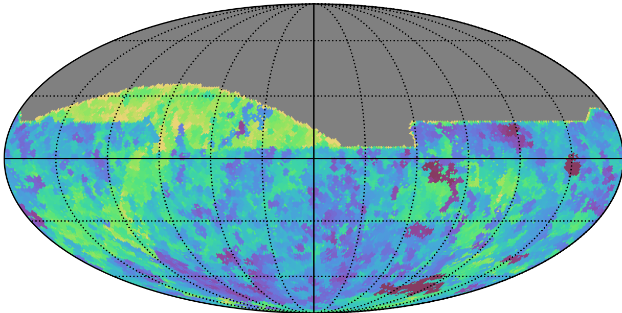
weather_cloudso35v3.4_10yrs All sky all bands: Min saturation_mag
