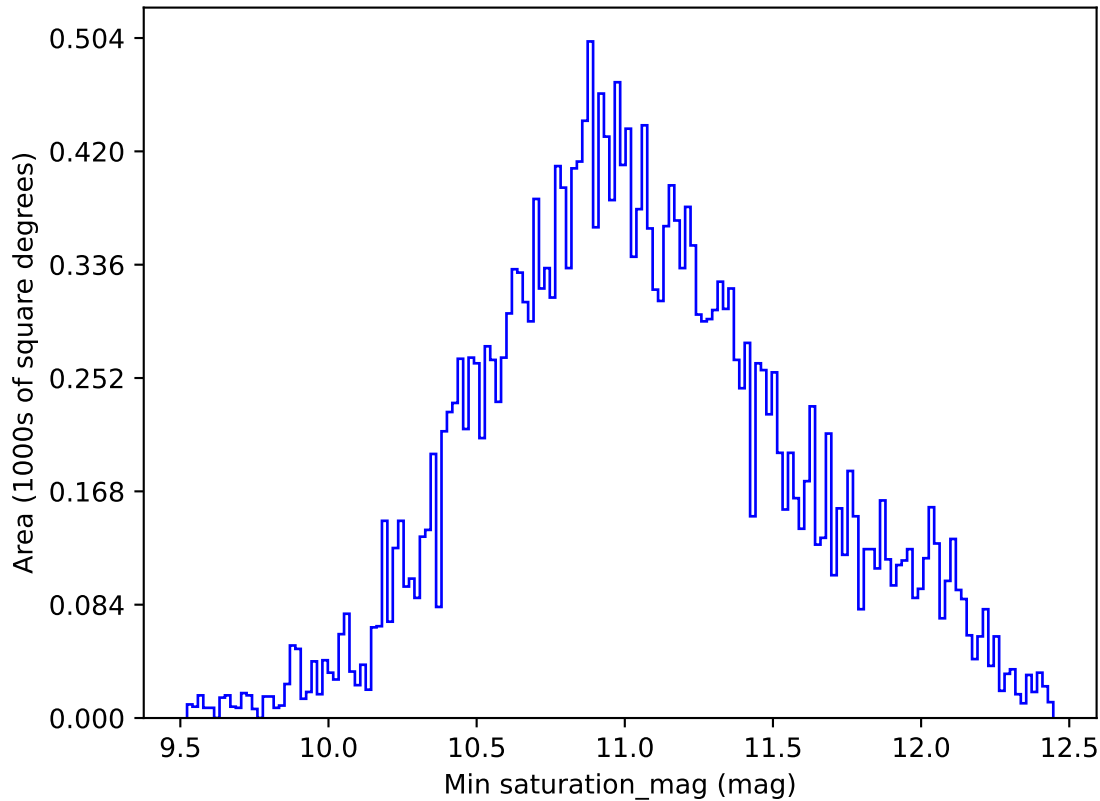
weather_cloudso35v3.4_10yrs All sky all bands: Min saturation_mag
