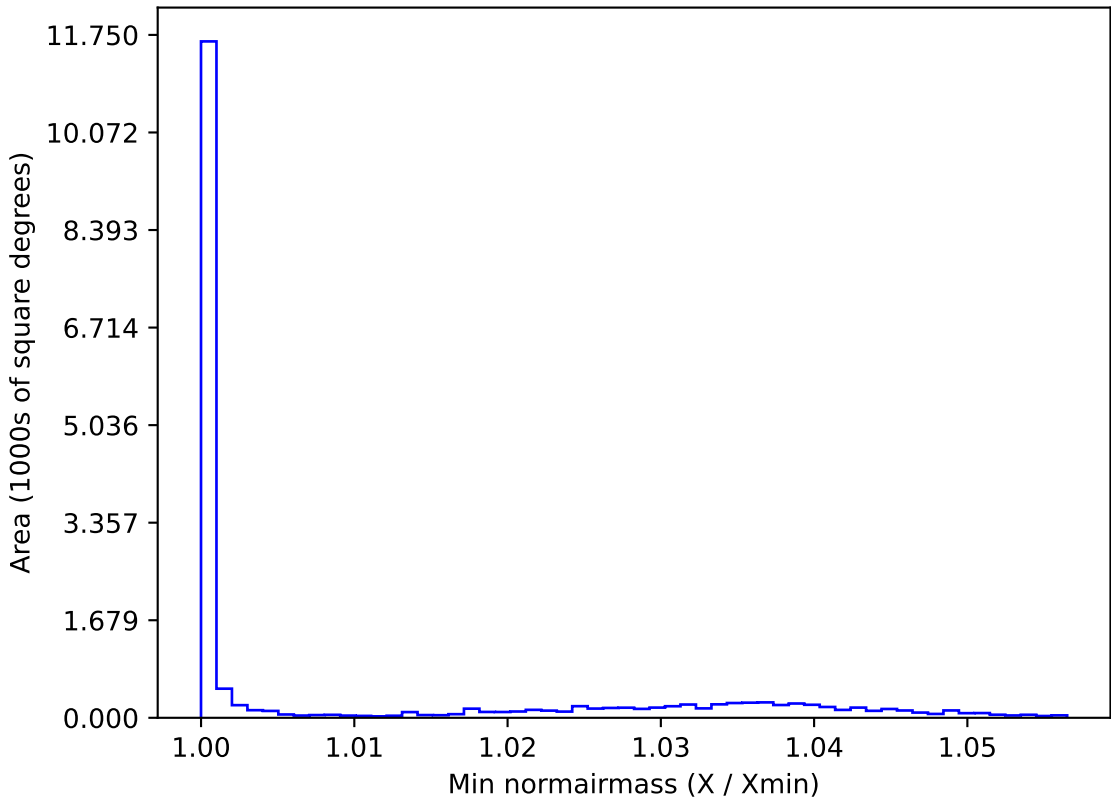
weather_cloudso35v3.4_10yrs WFD u band: Min normairmass
