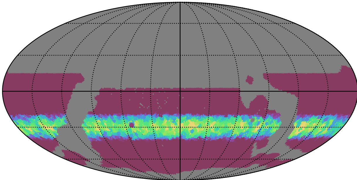
weather_cloudso35v3.4_10yrs WFD r band: Min normairmass
