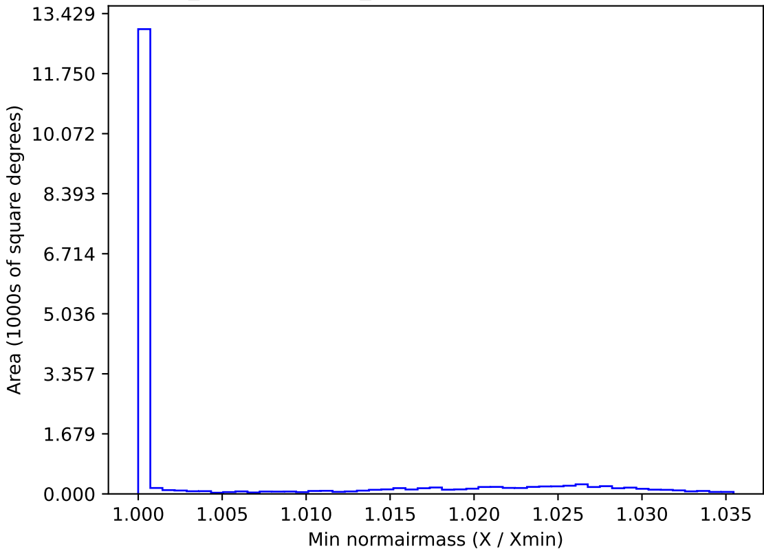
weather_cloudso35v3.4_10yrs WFD r band: Min normairmass
