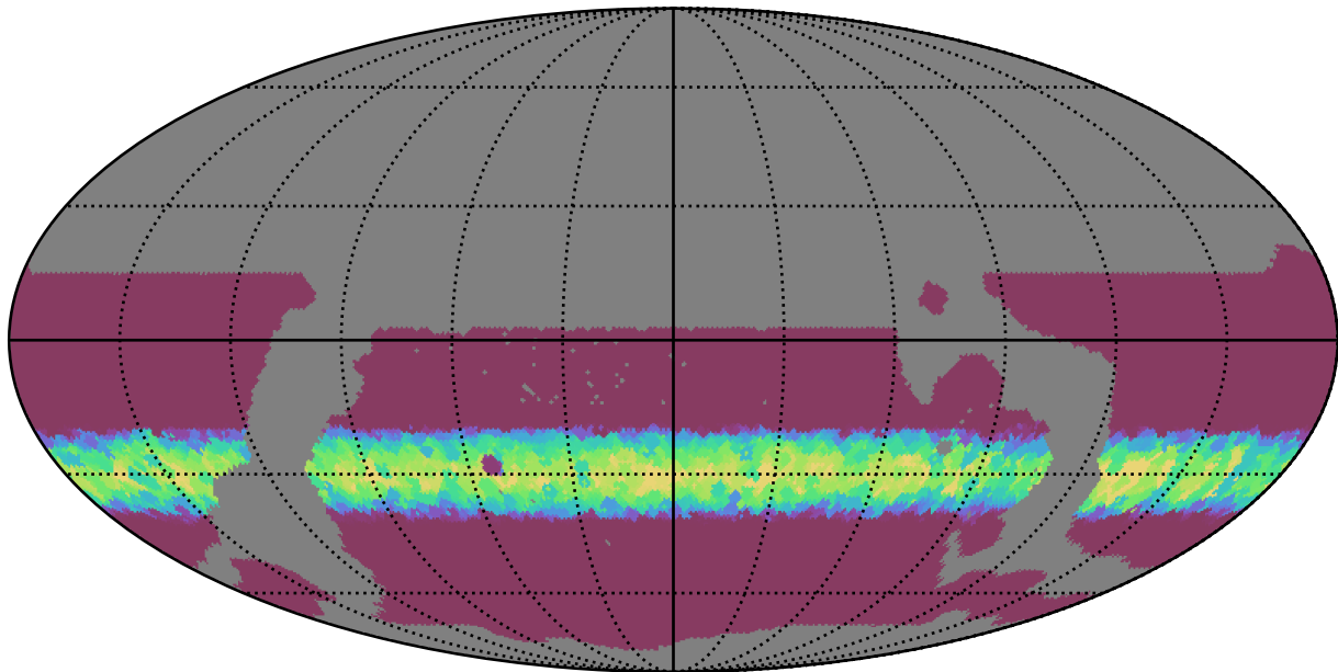
weather_cloudso35v3.4_10yrs WFD all bands: Min normairmass
