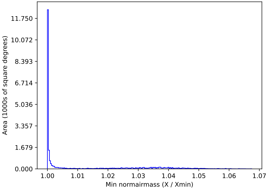
weather_cloudso35v3.4_10yrs All sky u band: Min normairmass
