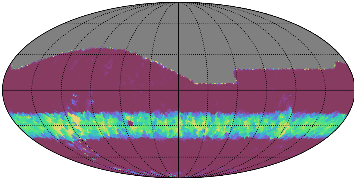
weather_cloudso35v3.4_10yrs All sky g band: Min normairmass
