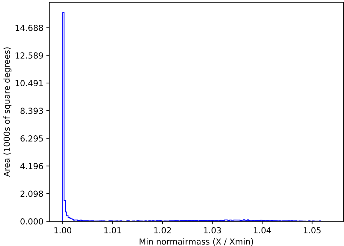
weather_cloudso35v3.4_10yrs All sky g band: Min normairmass
