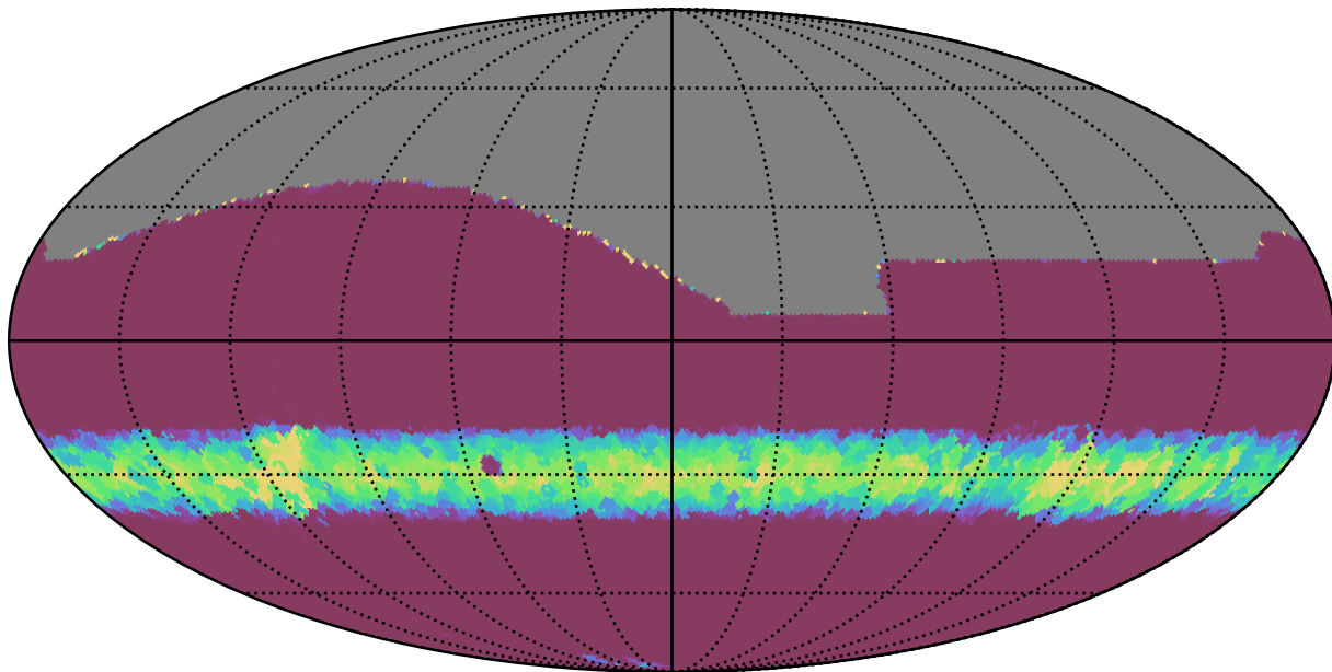
weather_cloudso35v3.4_10yrs All sky all bands: Min normairmass
