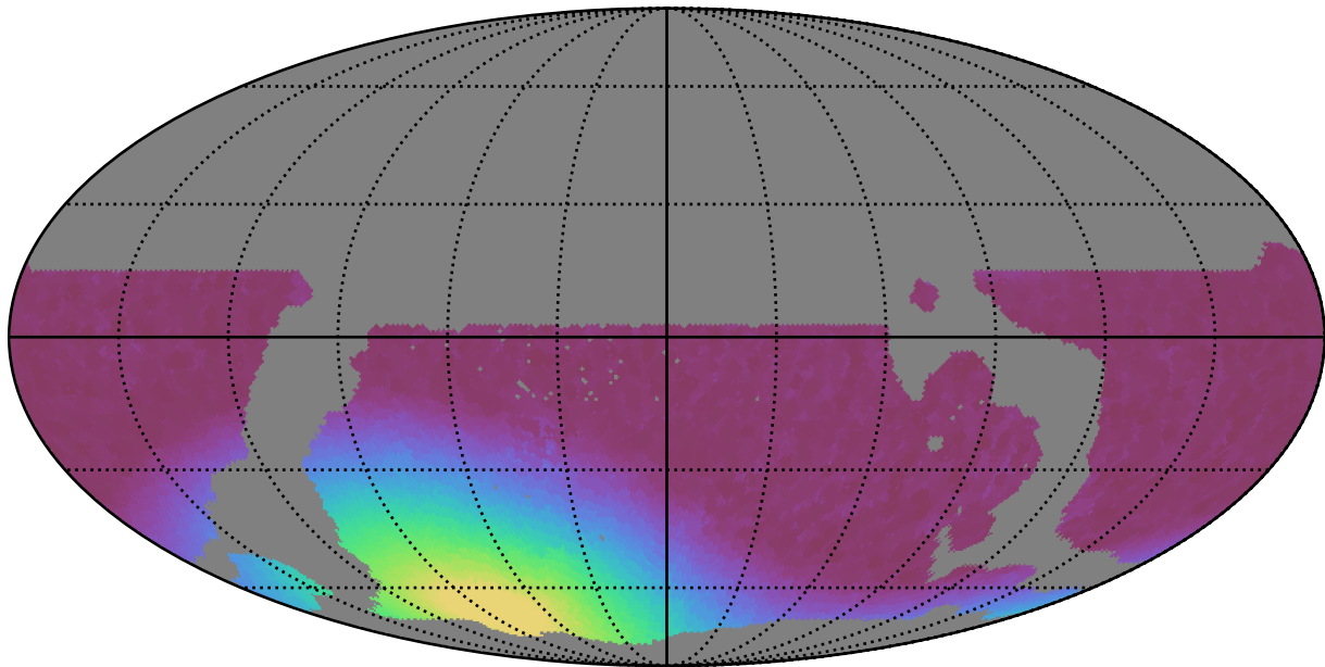
weather_cloudso35v3.4_10yrs WFD z band: Min moonDistance
