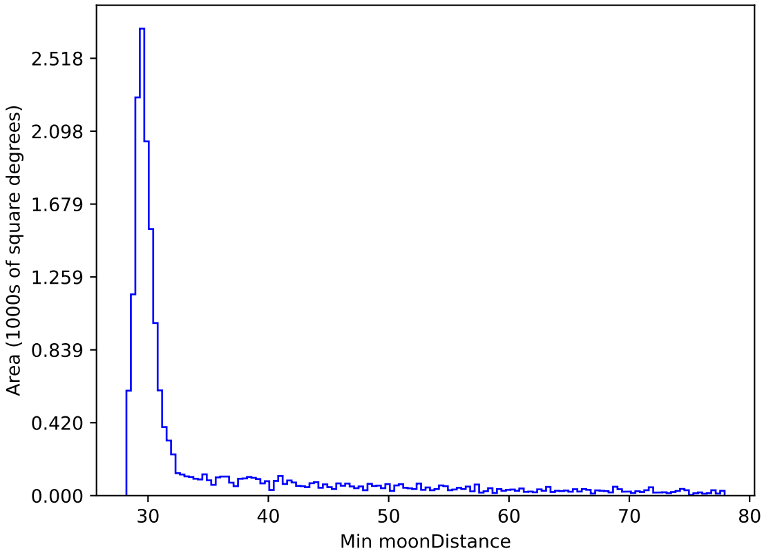
weather_cloudso35v3.4_10yrs WFD z band: Min moonDistance
